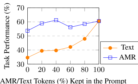
Figure 4: Ablation studies of AMR and text representations in the prompt on the AMR-NER dataset using GPT-4. Starting from the AMRCOT prompt with the complete text and AMR, we randomly drop out a certain portion of tokens in the text/AMR, and see the effect on the task performance.
