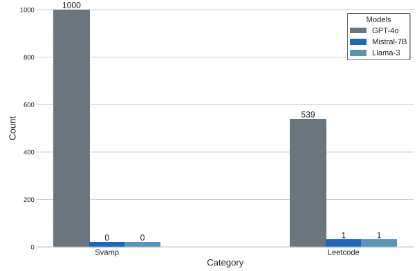
Figure 8: Routing results on Code and Math for SVAMP and LeetCode Subsets.
